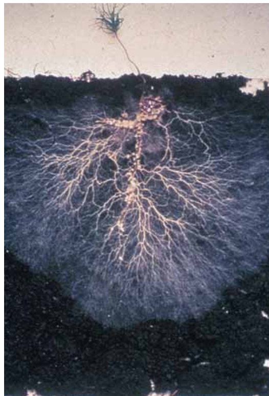
Mycorrhizal zone around roots of a pine seedling
